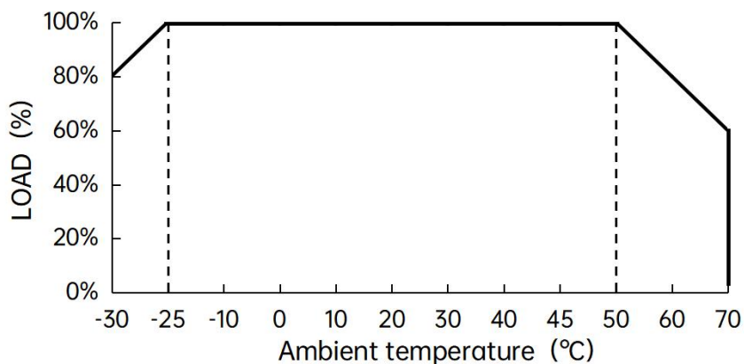
Ambient temperature VS Output power
