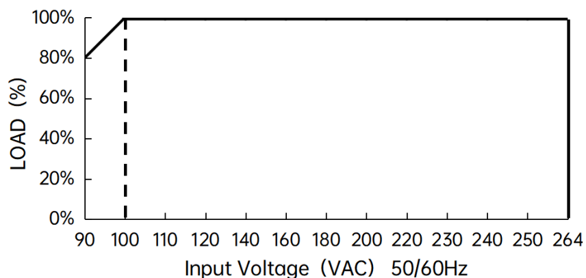
Input voltage VS Output power
