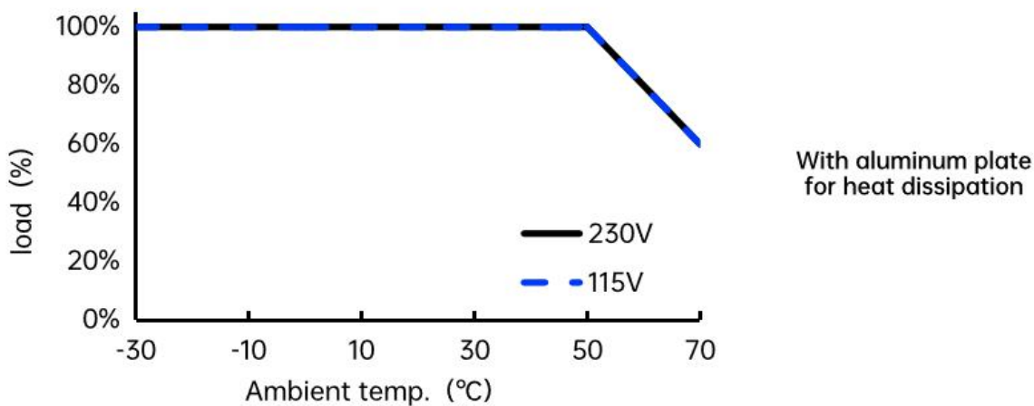
Ambient Temperature VS Output power
